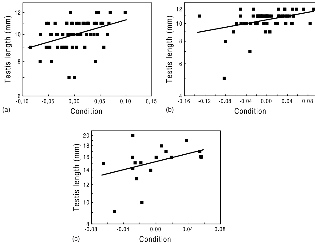
Fig. 1. Correlations with fitted regression lines between body condition (residual body mass) and testis size for (a) deer mice, (b) red-backed voles and (c) bushy-tailed woodrats. P < 0.05 for all three species. The y-axis is on a log 10 scale.
